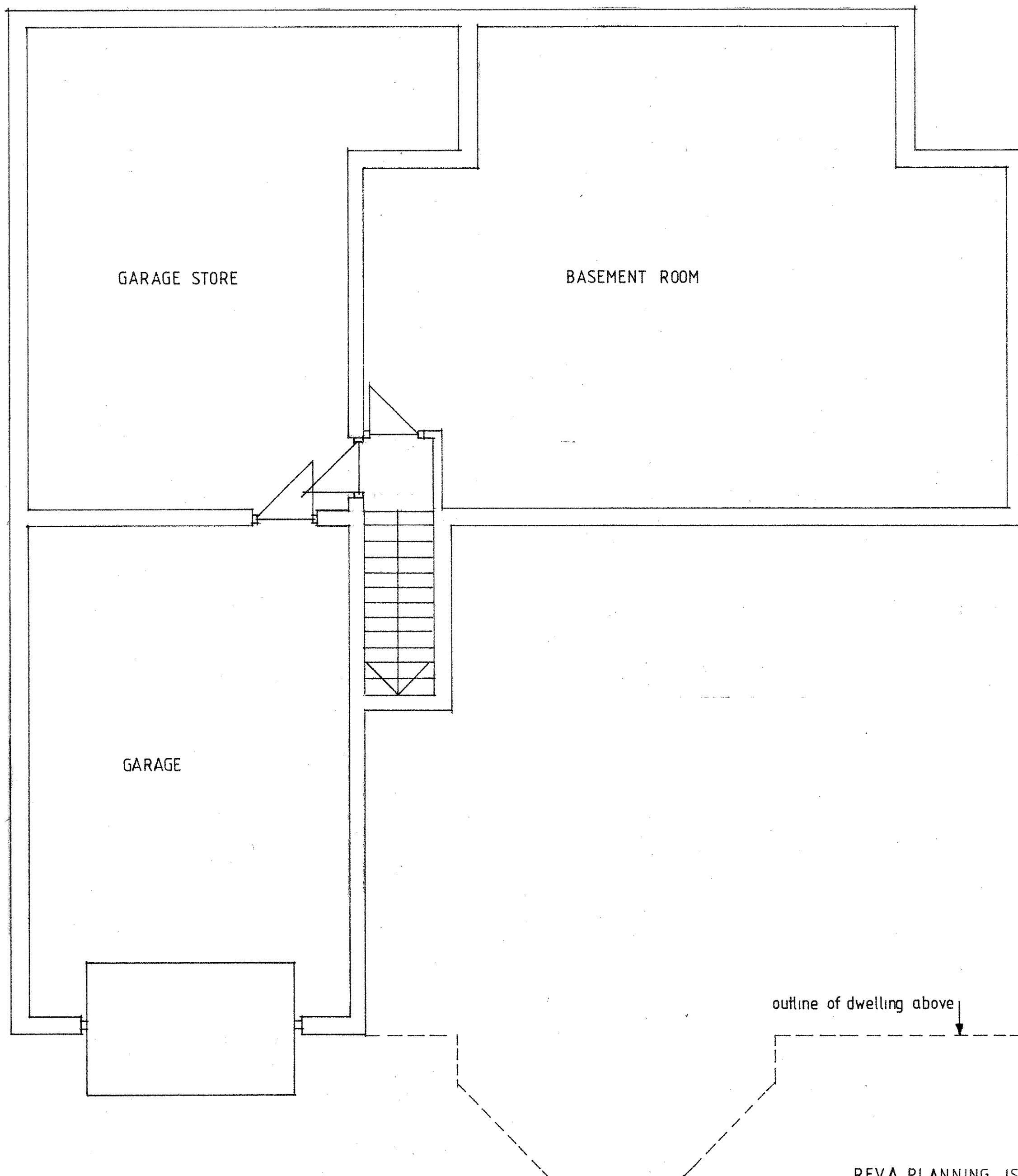
BASEMENT PLAN 1:50
